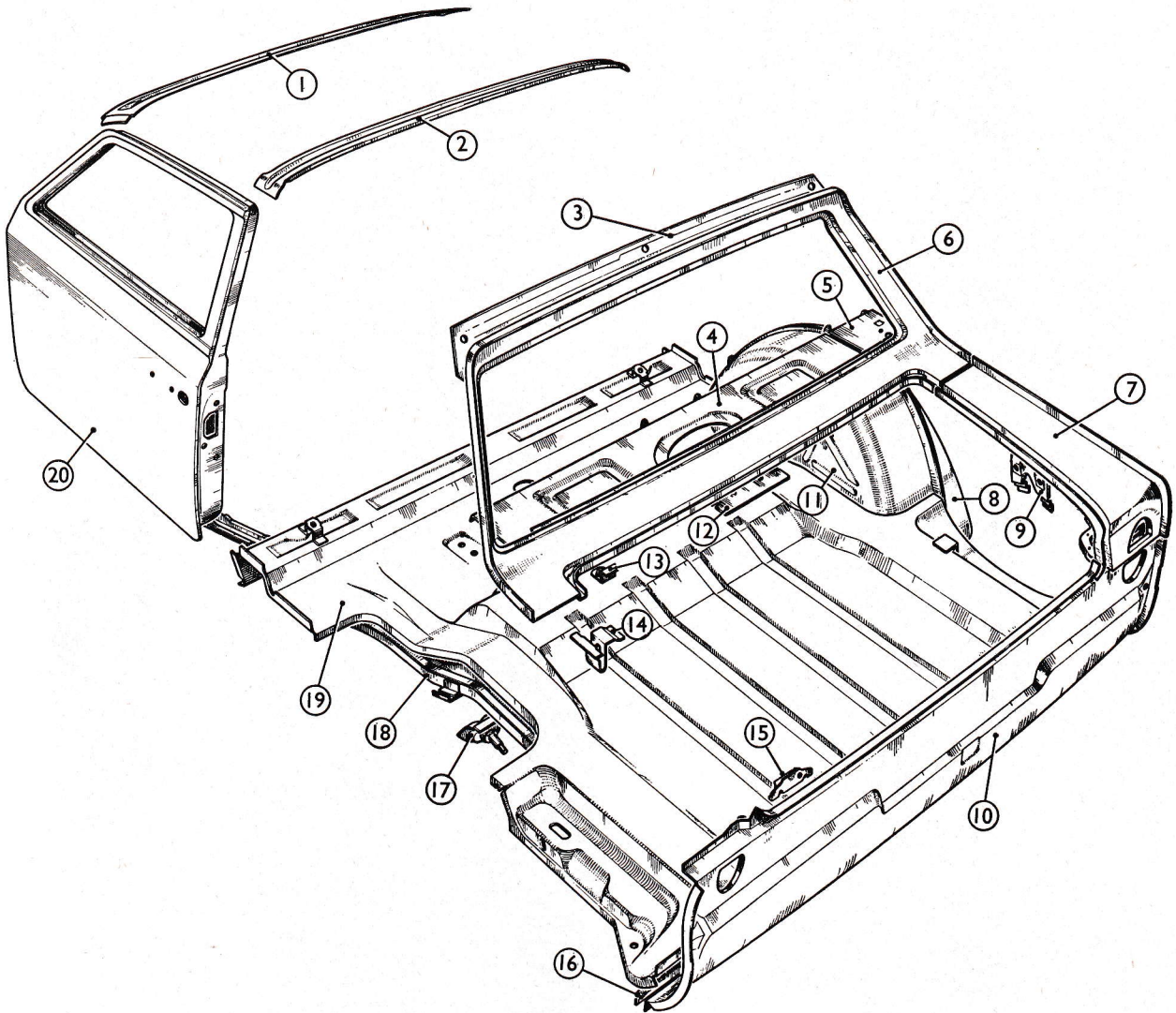
Fig. 98. Exploded view of body rear structure
